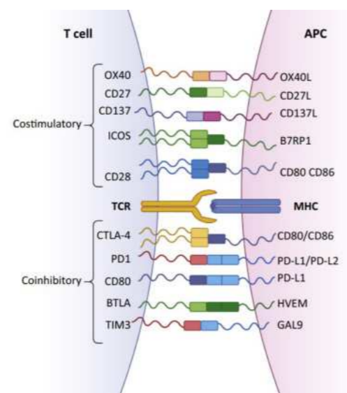
Co-stimulatory and co-inhibitory receptors in the immunological synapse [5]
